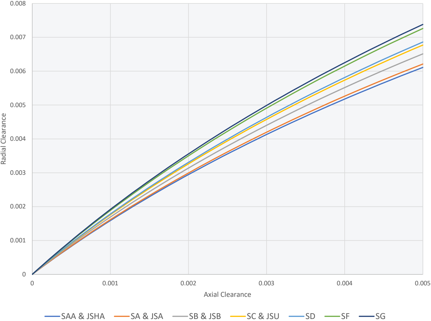
X-Type Radial vs Axial Clearance by Series
