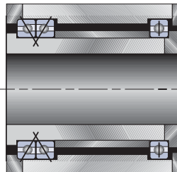
"A" Type "F" pair & floating "C" type mounting
