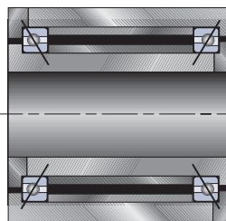
Face-to-Face mounting
